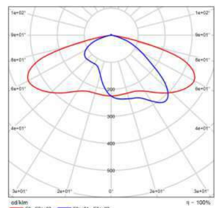
CDL polar
