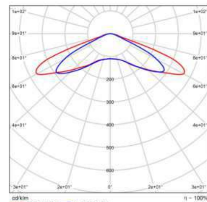
CDL polar
